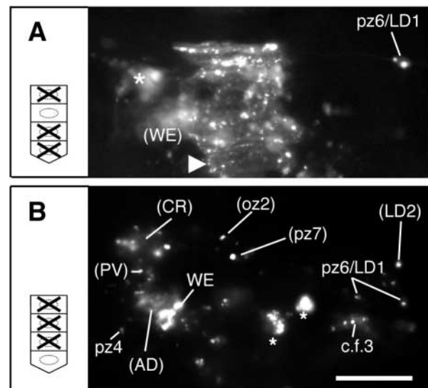
Fig. 6. Developmental regulation in ‘isolated’ P-type cells. (A) An example of an ‘isolated’ op 4 .ap cell clone. (B) An example of an ‘isolated’ op 4 .pp blast cell clone. In both cases, the ‘isolated’ P-type cell gives rise to pattern elements that are normally derived from the ablated sublineages (marked by parentheses) and unidentifiable cell clusters (marked by asterisks). Note that ‘isolated’ P-type cells give rise to a variable combination of pattern elements (see Table 1), and differing combinations were seen in different embryos. Scale bar: 20 μm.
