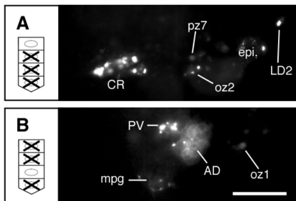
Fig. 5. ‘Isolated’ O-type cells show no sign of developmental regulation. (A) The ‘isolated’ op 4 .aa cell consistently gives rise to its normal fate (Fig. 3A). (B) The ‘isolated’ op 4 .pa cell consistently gives rise to its normal fate (Fig. 3F). Pattern element labels are given in Fig. 3. Scale bar: 20 μm.
