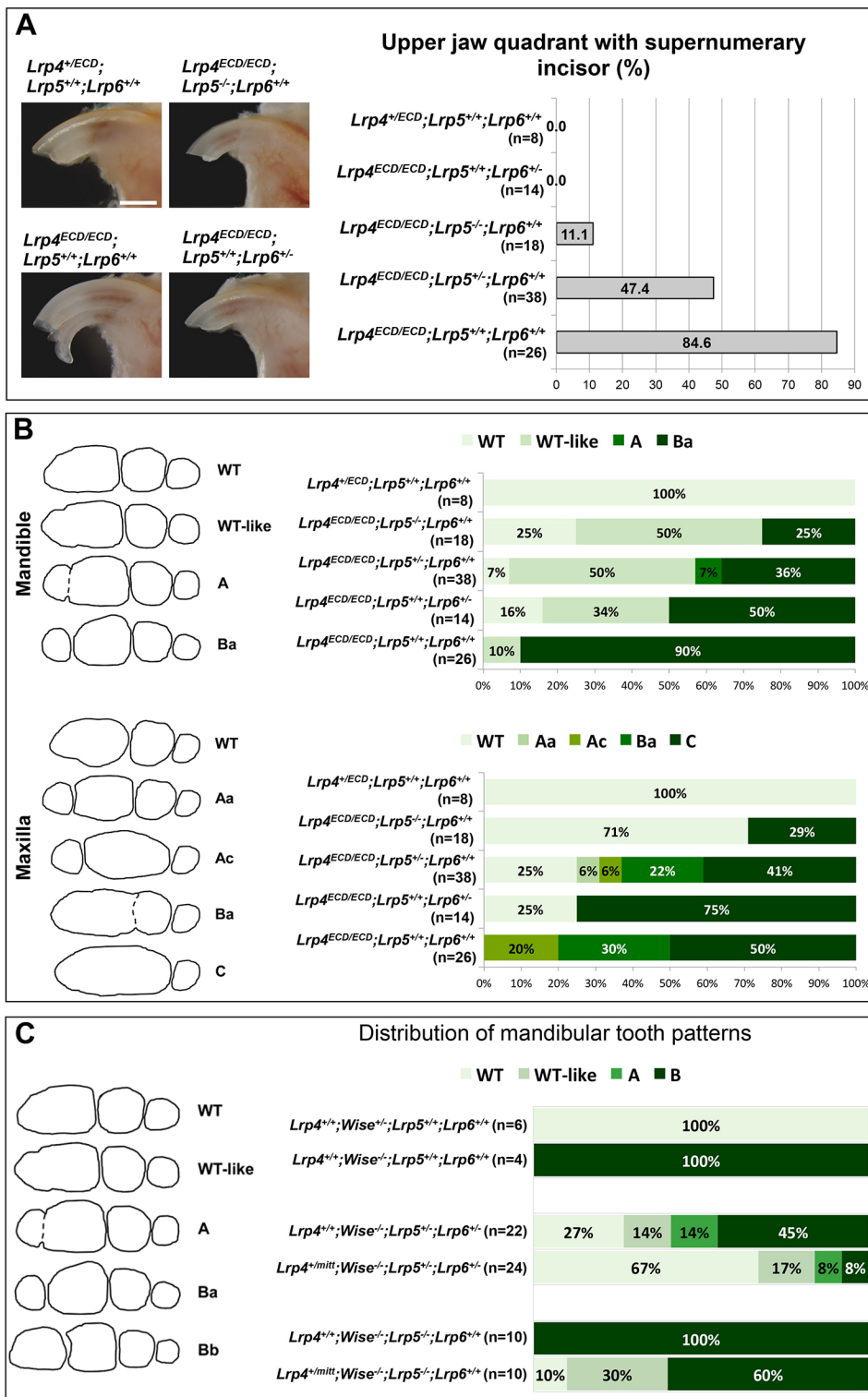
Fig. 3. Genetic interaction of Lrp4 with Lrp5 and Lrp6 in tooth development. (A) Reduced dosages of Lrp5 and Lrp6 rescue the supernumerary incisor phenotype of Lrp4 ECD/ECD mice. Scale bar: 1 mm. (B) Reduced dosages of Lrp5 and Lrp6 ameliorate molar abnormalities of Lrp4 ECD/ECD mice. (C) Reduced dosages of Lrp4 , Lrp5 and Lrp6 ameliorate Wise -null tooth defects in an additive manner.
