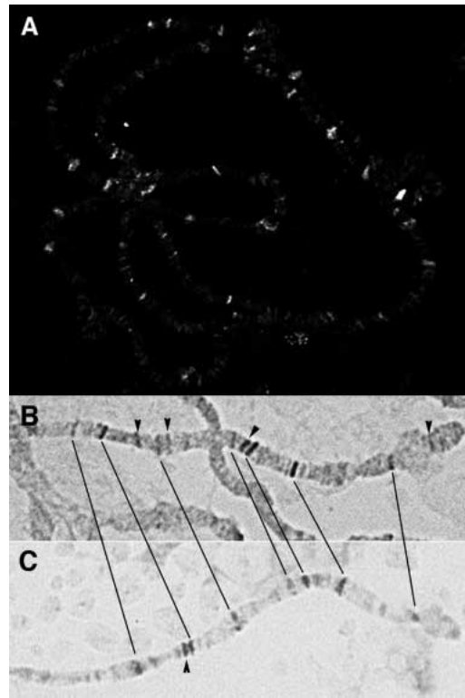
Fig. 6. ASX antibody staining of polytene chromosomes. (A) Sheep anti-peptide antibody on polytene nucleus from salivary gland. (B) ASX antibody staining of the distal portion of the X chromosome, compared to a similar region stained with PH antibody (C). Lines connect sites found with both antibodies and arrowheads mark unique binding sites.
