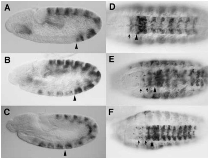
Fig. 5. Effects of Asx mutants on expression of bxdl-14 and Ubx . Embryos are mounted with anterior to the left and dorsal up and stained with antibodies (A-C) to \beta -galactosidase to detect activity of the bxdl4 reporter, or (D-F) to UBX to detect endogenous Ubx activity. The position of the border between parasegment 5 and 6 is marked with the arrowhead. Small arrows mark the positions of the parasegment 3-4 and 4-5 border, respectively. Embryos are homozygous for the Asx mutation and heterozygous for the bxdl4 reporter. Anti- \beta -galactosidase antibodies were used to monitor expression activity of the reporter. (A) Wild-type; (B) Asx P1 ; (C) Df(2R)trix ; (D) wild-type; (E) Asx 3 ; (F) Df(2R)trix .
