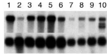
Fig. 3. Developmental northern analysis of Asx . The top panel was probed with the Asx cDNA. The bottom panel was probed with RP49 as a loading control. Poly(A) + RNA was prepared from 0-1.5 hour (lane 1); 1.5-3 hour (lane 2), 3-6 hour (lane 3), 6-9 hour (lane 4), 9-12 hour (lane 5), 12-18 hour (lane 6) embryos, mixed larvae (lane 7), pupae (lane 8), females (lane 9), and males (lane 10) respectively.
