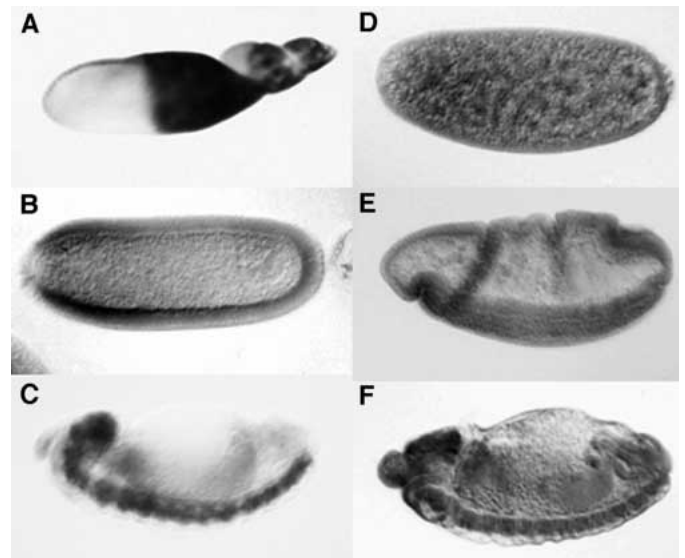
Fig. 4. Embryonic distribution of Asx mRNA and protein in oogenesis and embryogenesis. All embryos are mounted with anterior to the left and dorsal up. (A-C) RNA in situ. (A) Stage 10 oocytes; (B) cellular blastoderm embryo; note the increased hybridization in the anterior of the embryo; (C) stage 14 embryo, showing strong hybridization in the CNS; antibody staining; (D) stage 3 (preblastoderm) embryo; (E) stage 8 embryo; (F) stage 14 embryo.
