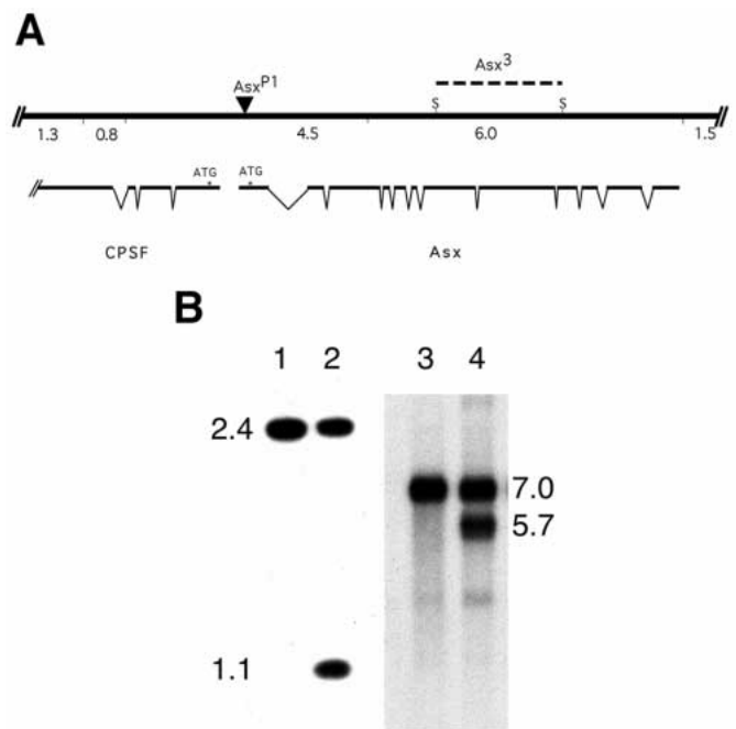
Fig. 1. Map of Asx locus, and mapping of Asx 3 mutation. (A) The thick black line indicates genomic DNA, with the telomere on the right. Sizes of Eco RI restriction fragments are indicated below. The triangle marks the insertion site of the P element responsible for the Asx P1 mutation. The dotted line above shows the approximate limits of the deletion associated with Asx 3 . Below are indicated the complete transcript of Asx , with locations of introns and the direction of transcription marked, and a partial cDNA of the proximal gene, which encodes dCPSF-160. (B) Southern and northern analyses of Asx 3 mutants. Lanes 1 (wild-type) and 2 ( Asx 3/+ ) show Southern analyses of genomic DNA cut with Sal I, and probed with the Asx cDNA, with size of bands indicated in kb at the left. Note the presence of a new band of 1.1 kb, corresponding to a 1.3 kb deletion in the Asx 3 mutation. Lanes 3 (wild-type) and 4 ( Asx 3/+ ) show northern analyses of embryonic poly(A) + RNA, with transcript sizes indicated on the right. Note the presence of a 5.7 kb RNA, corresponding to that expected from a 1.3 kb deletion in Asx .
