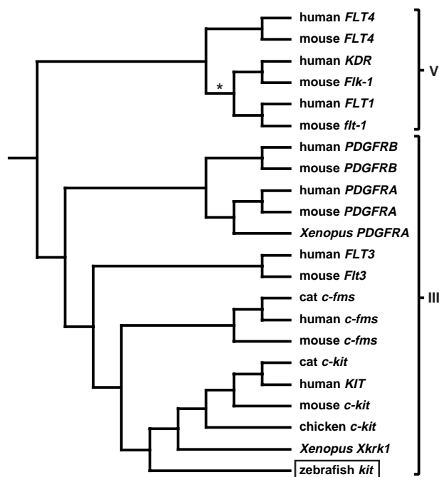
Fig. 2. Phylogenetic analysis demonstrates that zebrafish kit is orthologous to tetrapod kit genes. Shown is a maximum parsimony tree of selected type III and type V receptor tyrosine kinases, based on analyses of 2907 nucleotide positions of which 2890 were informative. Bootstrap support for all nodes was 100%, with the exception of the node leading to Flt-1 and KDR/Flk-1 genes (*), which was 94%. Analyses of nucleotide and amino acid sequences (not shown) both indicate that the zebrafish gene isolated here is more similar to kit -related genes of other taxa (including Xenopus Xkrk-1 ; Baker et al., 1995) than other type III receptor tyrosine kinases. Corresponding GenBank accession numbers from top to bottom in the figure are: 4503752; 293780; 3132832; 50976; 3132830; 2809068; 4505682; 53618; 189733; 200274; 214652; 406322; 50978; 163854; 29899; 50980; 913503; 4557694; 50423; 303532; 763033; 153446.
