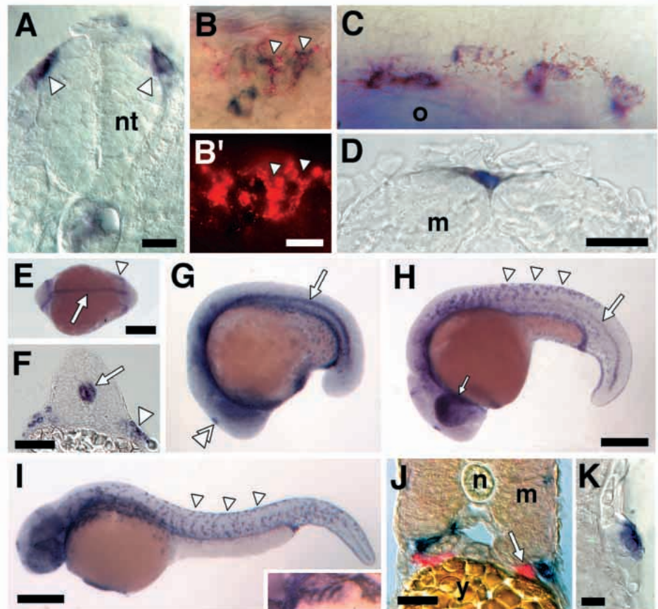
Fig. 3. kit is expressed by NC-derived melanoblasts and melanocytes during wild-type zebrafish development. (A) Transverse cryosection showing NC cells (arrowheads) expressing kit as they disperse from the neural tube (nt) (18 hours cryosection). (B) Two-color in situ hybridization reveals cells expressing both kit (blue, in B) and nacre (red, in B, B') in the dorsolateral NC migratory pathway (24 hours whole mount). (C) Lightly pigmented melanocytes expressing kit dorsal to the otocyst (o) (30 hours whole mount). (D) Fully differentiated melanocyte in the dorsal stripe expressing kit (12 day larva, cryosection); m, myotome (treated with PTU to partially inhibit melanin synthesis and better visualize kit staining). (E-K) kit also is expressed by an array of other cell types. (E) kit expression in notochord (arrow) and lateral mesodermal cells that are hematopoietic precursors and will form the intermediate cell mass (arrowhead; Detrich et al., 1995) (14 hours, whole mount dorsal view, anterior to left). (F) Notochord (arrow) and lateral mesodermal staining (arrowhead; 18 hours, transverse cryosection). (G) Notochord staining and staining in the pineal gland (double arrowhead; 17 hours, whole mount). (H) Dispersing, kit -expressing NC cells in the trunk (arrowheads), retinal staining in the eye (small arrow) and posterior notochord staining (large arrow; 22 hours, whole mount). (I) kit -expressing NC cells in the trunk (arrowheads) and branchial arches (inset; whole mount, 30 hours). (J) Zebrafish PGCs were not observed to express kit between 14 hours and 6.5 days. Shown are merged fluorescence and brightfield views of a transverse cryosection with vasa -stained PGCs (red) that do not stain for kit (blue, in adjacent melanocytes; 42 hours). n, notochord; y, yolk. (K) kit also is expressed in the lateral line sensory system (transverse cryosection, 3 day larva). In contrast to a Xenopus kit -like receptor (Baker et al., 1995) expressed in migrating lateral line primordia, zebrafish kit is expressed in differentiated sensory cells of lateral line neuromasts. Staining with DASPEI (Parichy, 1996a) does not reveal differences in midbody lateral line neuromast number between spa b5 and wild type ( F_{1,15}=0.77 , P=0.4 ). Scale bars: (A) 10 \mu m; (B) 5 \mu m; (C, D) 30 \mu m; (E) 500 \mu m; (F) 40 \mu m; (G, H) 500 \mu m; (I) 250 \mu m; (J) 30 \mu m; (K) 10 \mu m.
