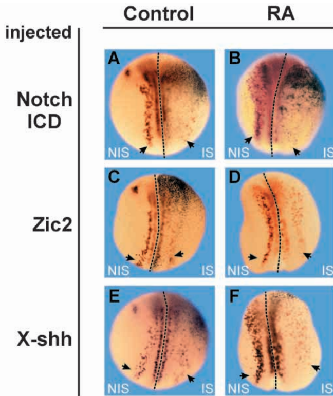
Fig. 4. RA acts upstream of lateral inhibition, Zic2 and X-shh in the primary neurogenesis cascade. Embryos were coinjected unilaterally with 100 pg nuc-β-gal mRNA as tracer plus Notch ICD , Zic2 or X-shh mRNAs and left untreated (control column) or treated with RA during gastrulation (RA column). N-tubulin distribution was revealed by in situ hybridization at neurula stage. All are dorsal views (anterior up). Dotted line, dorsal midline; IS, injected side (blue staining); NIS, non-injected side. Sensory neuron stripes are marked with arrows. Percentages below indicate the reduction of N-tubulin expression in the IS. (A,B) RA treatment cannot overcome the inhibitory effect of Notch ICD on N-tubulin expression. Notch ICD -injected embryos, untreated (A, 93%, n =11 for 1 ng Notch ICD ; 75%, n =14 for 0.5 ng Notch ICD ). Notch ICD -injected embryos, treated with RA (B, 100%, n =10 for 1 ng Notch ICD + 10 μM RA; 70%, n =10 for 1 ng Notch ICD + 1 μM RA; 73%, n =11 for 0.5 ng Notch ICD + 10 μM RA; 100%, n =10 for 0.5 ng Notch ICD + 1 μM RA). (C,D) RA treatment cannot rescue the inhibitory effect of Zic2 on N-tubulin expression. Zic2 -injected embryos, untreated (C, 20%, n =22 for 2 ng Zic2 ; 15%, n =32 for 1 ng Zic2 ). Zic2 -injected embryos, treated with RA (D, 22%, n =23 for 1 ng Zic2 + 10 μM RA). (E,F) RA treatment cannot rescue the inhibitory effect of X-shh on N-tubulin expression. X-shh -injected embryos, untreated (E, 17%, n =6 for 0.25 ng X-shh ). X-shh -injected embryos, treated with RA (F, 30%, n =10 for 0.25 ng X-shh + 10 μM RA). All RA-treated embryos showed the previously described enhancement of N-tubulin expression in the uninjected side.
