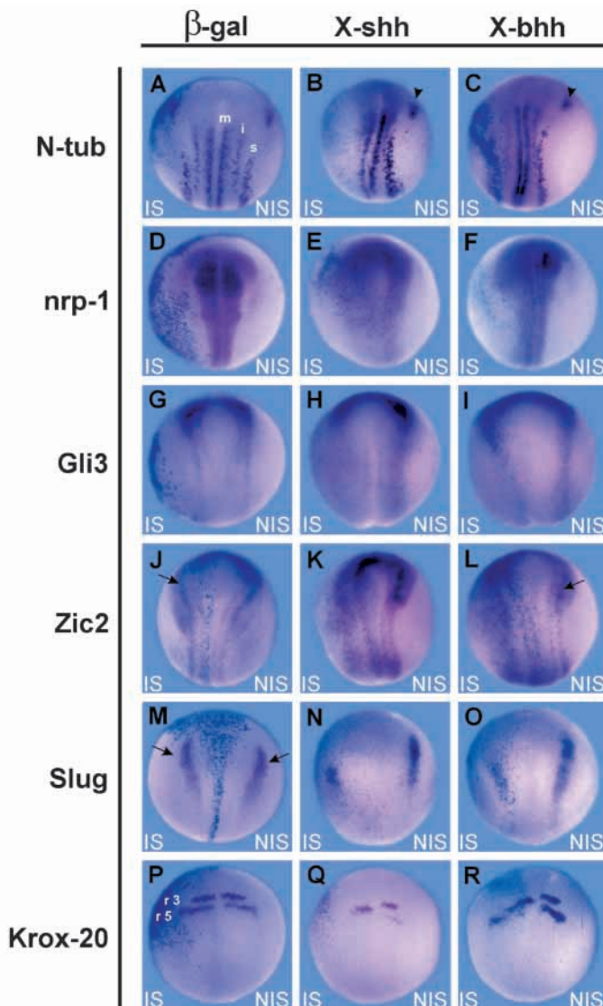
Fig. 2. X-shh and X-bhh overexpression increased the expression of inhibitors and repressed the expression of activators of primary neurogenesis, and reduced neural crest markers without impairing neural development. Embryos were unilaterally injected with 1 or 2 ng of nuc-β galactosidase mRNA as a negative control ( β-gal column), full-length X-shh mRNA ( X-shh column) or full-length X-bhh mRNA ( X-bhh column) plus 100 pg of nuc-βgal mRNA as tracer. They were analyzed at neurula stage by whole-mount in situ hybridization with different neural markers. All are dorsal views (anterior up). The injected side is demarcated by the pale blue staining and is oriented to the left. IS, injected side. NIS, non-injected side. (A-C) Suppression of primary neuron formation as revealed by the differentiation marker N-tubulin ( N-tub ) in X-shh -injected embryos (B, 90%, n=21 for 2 ng; 79%, n=14 for 1 ng; 57%, n=21 for 0.125 ng) and X-bhh -injected embryos (C, 100%, n=24 for 2 ng; 93%, n=14 for 1 ng; 28%, n=22 for 0.125 ng). Notice the absence of N-tubulin expression from the trigeminal ganglion in the injected side. m, i and s, primary motor neurons, interneurons and sensory neurons, respectively; arrowhead, trigeminal ganglion. (D-F) Expansion of the neural plate as revealed by the general neural marker nrp-1 in X-shh -injected embryos (E, 100%, n=10 for 2 ng) and X-bhh -injected embryos (F, 100%, n=10 for 2 ng). (G-I) Abolishment of Gli3 expression in the posterior neural plate in X-shh -injected embryos (H, 67%, n=21 for 2 ng; 15%, n=13 for 1 ng) and X-bhh -injected embryos (I, 50%, n=26 for 2 ng). Notice that nuc-βgal dark-blue staining may interfere with the appreciation of Gli3 decrease on the injected side. (J-L) Widespread expansion of Zic2 domain in X-shh -injected embryos (K, 71%, n=34 for 2 ng; 44%, n=18 for 0.25 ng) and X-bhh -injected embryos (L, 80%, n=35 for 2 ng; 32%, n=63 for 0.25 ng). Notice the absence of Zic2 expression from the medial cranial neural crest domain (arrow) in the injected side. (M-O) Reduction and ventral displacement of the Slug domain in X-shh -injected embryos (N, 82%, n=22 for 2 ng; 64%, n=11 for 1 ng; 35%, n=17 for 0.25 ng) and X-bhh -injected embryos (O, 50%, n=6 for 1 ng; 32%, n=25 for 0.25 ng). Arrows, neural crests. (P-R) Downregulation of Krox-20 in r5 and caudal displacement of r3 domain in X-shh -injected embryos (Q, 60%, n=10 for 2 ng) and X-bhh -injected embryos (R, 60%, n=10 for 2 ng). r3, third rhombomere; r5, fifth rhombomere.
