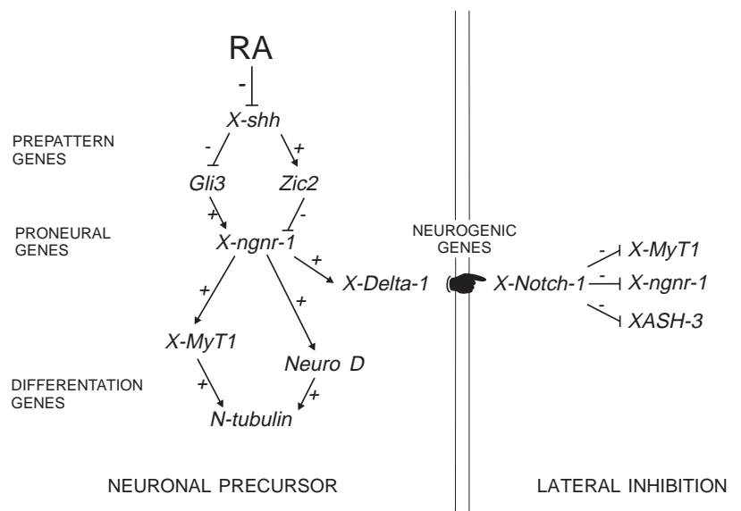
Fig. 5. Proposed model for the molecular interactions involving RA and hedgehog signaling leading to terminal primary neuronal differentiation.
