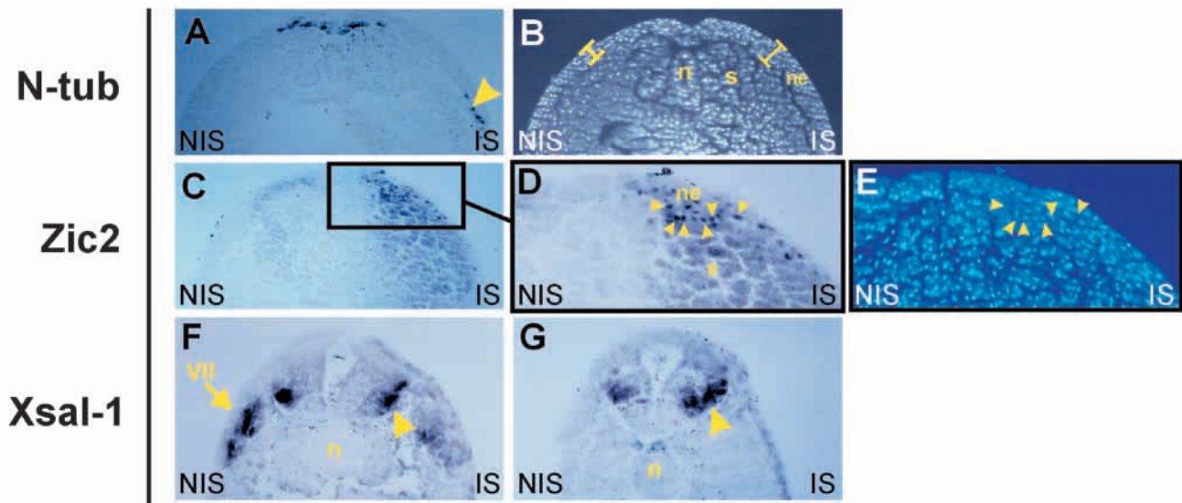
Fig. 3. Cross sections of X-shh - and X-bhh -injected embryos at neurula stage (A-E) and tadpole stages (F,G). Dorsal side is up. IS, injected side; NIS, non-injected side; n, notochord; ne, neural ectoderm; s, somites. (A) N-tubulin distribution shows the ventral displacement of the primary sensory neurons stripe (arrowhead) in the IS. (B) Hoechst nuclear labeling revealing the increased cell number in the IS including the neural ectoderm (compare bars). (C,D) Zic2 expression. Note the expansion in the neural ectoderm and mesoderm in the IS in C. The inset shown at higher magnification in D shows the very active transcription of Zic2 in nuclei (arrowheads) of the IS. (E) The same section as in D revealed for Hoescht staining, confirms the nuclear location (arrowheads) of Zic2 transcripts. (F,G) Xsal-1 expression is downregulated in the VII th cranial ganglion (arrow in F) and reveals an expansion of ventral secondary neurons within the neural tube (arrowheads in F and G) in the IS.
