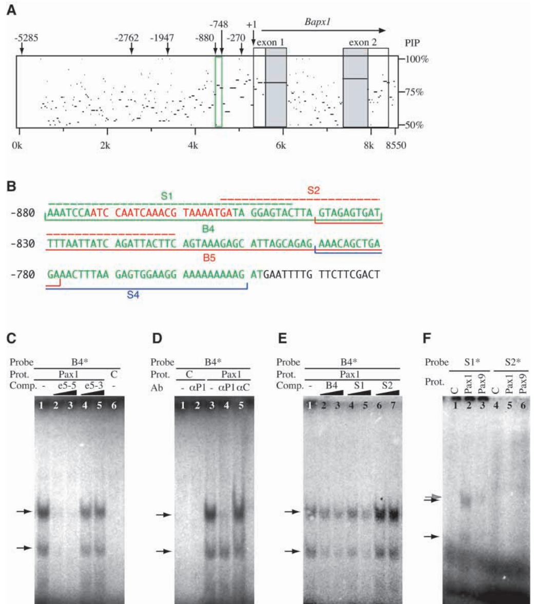
Fig. 7. Pax1 and Pax9 bind to regulatory sequences of the Bapx1 promoter. (A) PIP analysis of an 8550 bp mouse Bapx1 genome sequence when compared with an 8600 bp human BAPX1 sequence. Exons are outlined in black and coding parts are gray. Numbers at the top indicate nucleotide positions as defined in the text, and they correspond to 5' ends of intervals included in the series of deletion constructs used in the transactivation assay. The interval between -880 and -748 is outlined in green. PIP scores in % are shown on the right, with 50% identity at the bottom level. Note the presence of several CNS segments outside the coding region. Many of them are located in the interval between -880 and +109. (B) Sequence of the interval between -880 and -731. The different oligonucleotides (S1, S2, B4, B5 and S4) employed in EMSA assays are indicated by lines. Sequence in green (-880 to -748) corresponds to the segment included in the plasmid p0.9Bp-luc, but not in the plasmid p0.7Bp-luc. A potential Pax6-binding site predicted by TFSEARCH and MatInspector is in the region of S1 and indicated in red. (C-F) Results of EMSA experiments. The indicated labeled oligonucleotides (Probe, marked with an asterisk) were incubated with the in vitro translated protein (Prot.) Pax1, Pax9 or luciferase as a control (C), separated and visualized as described in the Materials and Methods. The specific Pax1 (black arrows) and Pax9 (gray arrow in F) complexes are indicated. (C) Pax1 binds to oligonucleotide B4. Cold oligonucleotides e5-5 or e5-3 were added at 250-fold (lanes 2, 4) or 500-fold (lanes 3, 5) molar excess, as indicated. e5-5 specifically competes with B4 for Pax1 binding, whereas mutated e5-3 does not. (D) Specific inhibition of Pax1-B4 complex formation by anti-Pax1 antibody. The indicated antibodies were incubated in the binding reactions. \alpha P1, anti-Pax1 goat antibody; \alpha C, anti-mouse goat antibody, used as control. The anti-Pax1 antibody abrogates the formation of the larger complex. (E) Competition experiments employing a 250-fold (lanes 2, 4, 6) or 500-fold (lanes 3, 5, 7) molar excess of cold oligonucleotides B4, S1 or S2. Note that oligonucleotides B4 and S1 compete with B4 for Pax1 binding, whereas oligonucleotide S2 does not. (F) Binding of Pax1 and Pax9 to oligonucleotide S1. S1 or S2 labeled oligonucleotides were incubated with Pax1, Pax9 or luciferase control protein as indicated. Both Pax1 and Pax9 interact with S1 oligonucleotide, but not with S2 oligonucleotide.
