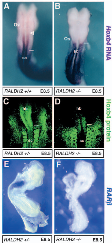
Fig. 2. Early hindbrain expression of Hoxb4 and Rarb requires Raldh2 activity. The effects of loss of Raldh2 activity on the early neural expression of Hoxb4 mRNA (A,B), Hoxb4 protein (C,D) and Rarb gene (E,F) are shown. (A,B) Dorsal views of E8.5 embryos showing the Hoxb4 mRNA distribution in Raldh2 +/+ (A) and Raldh2 -/- (B) genetic backgrounds. Loss of Raldh2 function is associated with absence of Hoxb4 mRNA within the hindbrain but expression within the developing spinal cord (sc) remains unaffected. (C,D) Dorsal views of E8.5 embryos showing Hoxb4 protein expression in Raldh2 +/+ (C) and Raldh2 -/- (D) embryos. Removal of Raldh2 activity leads to loss of most Hoxb4 protein within both the developing hindbrain (hb) and spinal cord (sc). However, weak expression is still observed within a few cells at caudal hindbrain and anterior spinal levels. (E,F) Rarb mRNA induction within the hindbrain requires Raldh2 activity. Lateral views of E8.5 embryos of the genotypes Raldh2 +/+ (E) or Raldh2 -/- (F). Loss of Raldh2 activity is associated with the absence of all detectable Rarb expression within the developing hindbrain and spinal cord. Os and Ov indicate the otic sulcus and otic vesicle, lying adjacent to r5 and r6 in this and subsequent figures, and the approximate position of the paraxial mesodermal limit of Hoxb4 expression at the somite 6/7 border is also shown (horizontal line in A-D).
