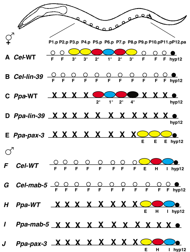
Fig. 1. Schematic summary of ventral epidermal cell fate specification in P. pacificus and C. elegans wild-type and mutant animals. The ventral epidermis of hermaphrodites and males derives from 12 ectoblasts, named P(1-12).p according to their anteroposterior position. The 12 cells are equally distributed between the pharynx and rectum. (A-E) Cell fate specification in the hermaphrodite. (A) C. elegans wild-type. The vulva is formed from the progeny of the 1° (blue ovals) and 2° (red ovals) vulva precursor cells. 3° cells (yellow ovals) are competent to form vulval tissue, but remain epidermal under wild-type conditions. In C. elegans , P(1,2,9-11).p fuse ('F', white circles) with the hypodermis and are not competent to form part of the vulva. P12.pa is a special cell called hyp12 and forms part of the rectum. (B) In C. elegans lin-39 mutants, positional information for the formation of the vulva equivalence group is missing and P(3-8).p fuse with the hypodermis, as do their lineage counterparts in the anterior and posterior body region. (C) In P. pacificus , P(1-4,9-11).p die as a result of programmed cell death (X) and reduce the size of the vulva equivalence group further. P(5-7).p have a 2°-1°-2° pattern, as is also observed in C. elegans , and P8.p is a special epidermal cell (black oval), which is designated as a 4° cell fate. (D) In Ppa-lin-39 mutants, the vulva equivalence group is not formed and P(5-8).p die as a result of programmed cell death ('X'). (E) The Ppa-pax-3 mutants have opposite effects on the Pn.p cells in the central and the posterior body region: P(5-8).p undergo ectopic cell death, whereas P(9-11).p often survive. 'E' denotes epidermal cell fate. (F-J) Cell fate specification in males. (F) In C. elegans , P(1-8).p fuse (white circles) with the hypodermis. P10.p and P11.p divide multiple times and form the hook ('H') and associated interneurons ('I'). P9.p remains epidermal, but has been shown to be able to replace P10.p after cell ablation of the latter. (G) In Cel-mab-5 mutants, P(9-11).p fuse with the hypodermis, and no hook is formed. (H) In P. pacificus , P(1-8).p undergo programmed cell death and P(9-11).p development resembles the pattern observed in C. elegans . (I) In Ppa-mab-5 mutants, P(1-11).p die as a result of programmed cell death, suggesting that mab-5 provides positional information for P(9-11).p specification in both species. (J) In Ppa-pax-3 mutants, no patterning differences are observed.
